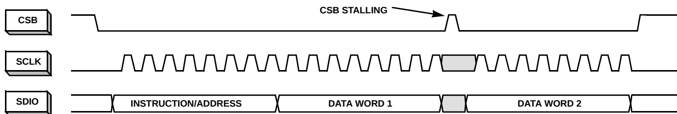
FIGURE 39. SPI READ
