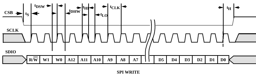
FIGURE 38. SPI WRITE
