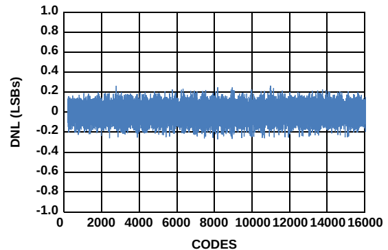
FIGURE 12. DIFFERENTIAL NONLINEARITY
