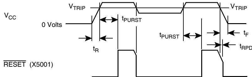
Figure 12. Power-Up and Power-Down Timing
