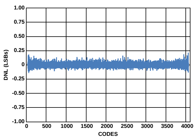
FIGURE 12. DIFFERENTIAL NONLINEARITY (250MSPS)
