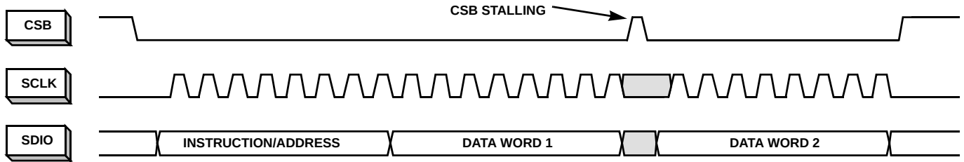
FIGURE 58. 2-BYTE TRANSFER
