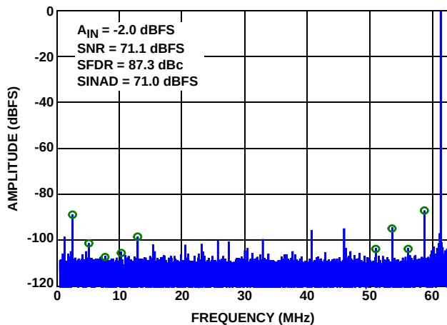
FIGURE 23. SINGLE-TONE SPECTRUM @ 190MHz (125MSPS)
