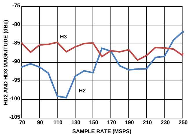
FIGURE 10. HD2 AND HD3 vs f_{SAMPLE}
