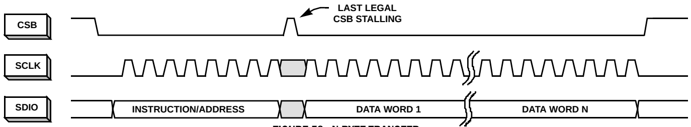
FIGURE 59. N-BYTE TRANSFER
