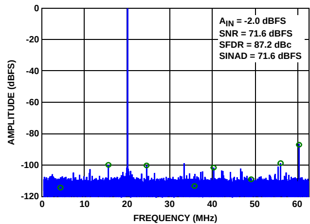
FIGURE 22. SINGLE-TONE SPECTRUM @ 105MHz (125MSPS)
