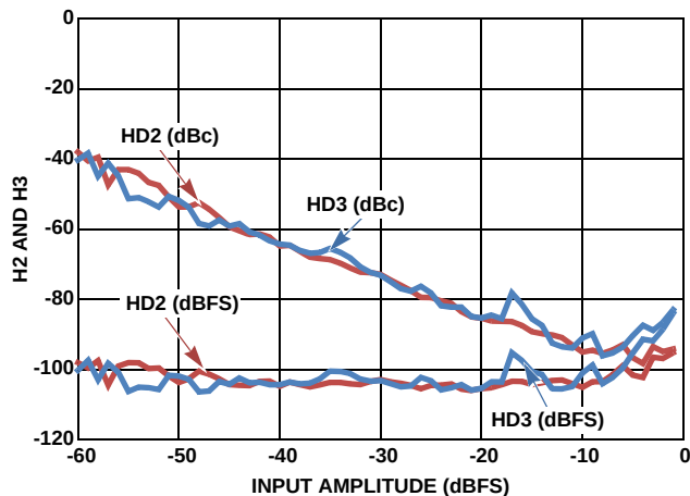
FIGURE 8. H2 AND H3 vs A_{IN} (125MSPS)
