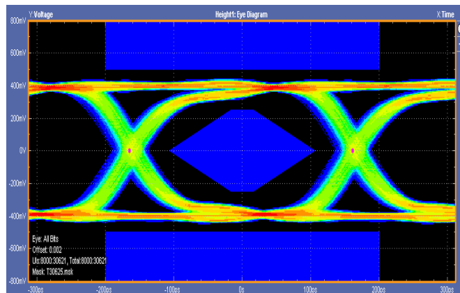
FIGURE 28. SERDES DATA EYE at 3.0Gbps
