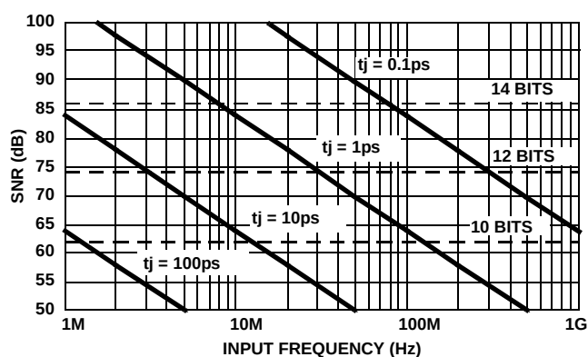
FIGURE 49. SNR vs CLOCK JITTER
