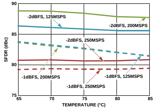
FIGURE 43. TYPICAL SFDR PERFORMANCE vs TEMPERATURE, DEVICE CALIBRATED AT +85^{\circ}\text{C} , f_{\text{IN}} = 105\text{MHz}
