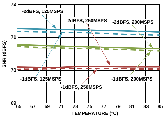
FIGURE 42. TYPICAL SNR PERFORMANCE vs TEMPERATURE, DEVICE CALIBRATED AT +85^{\circ}\text{C} , f_{\text{IN}} = 105\text{MHz}
