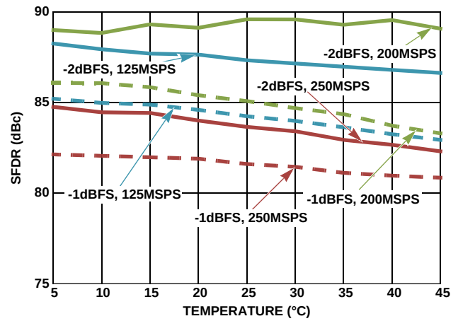
FIGURE 41. TYPICAL SFDR PERFORMANCE vs TEMPERATURE, DEVICE CALIBRATED AT +25^{\circ}\text{C} , f_{\text{IN}} = 105\text{MHz}
