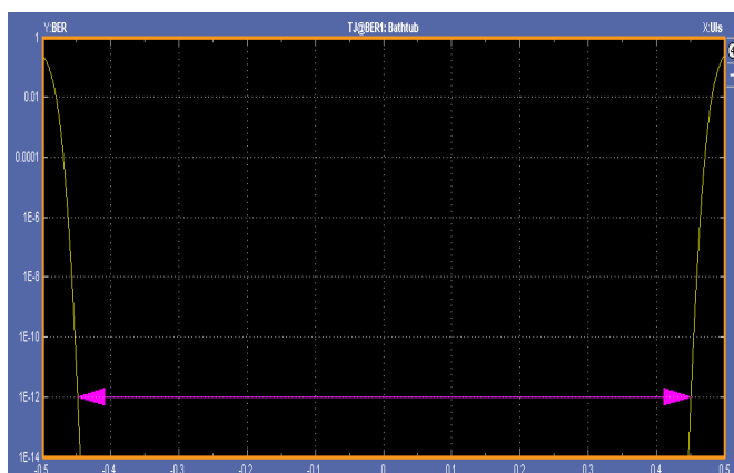
FIGURE 30. SERDES BATHTUB at 1.0Gbps
