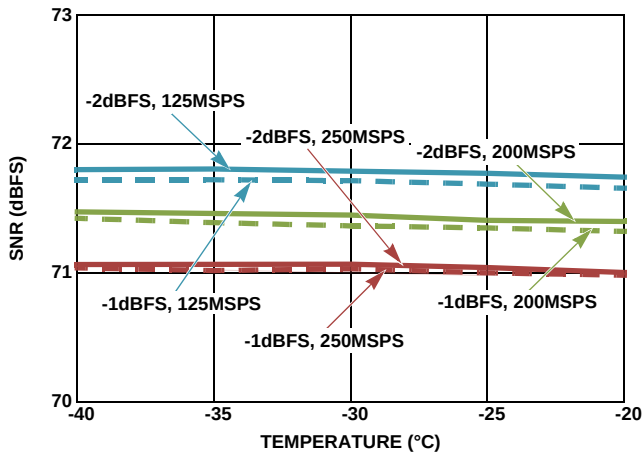
FIGURE 38. TYPICAL SNR PERFORMANCE vs TEMPERATURE, DEVICE CALIBRATED AT -40^{\circ}\text{C} , f_{\text{IN}} = 105\text{MHz}
