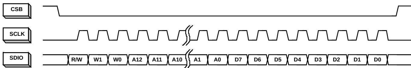
FIGURE 54. MSB-FIRST ADDRESSING
