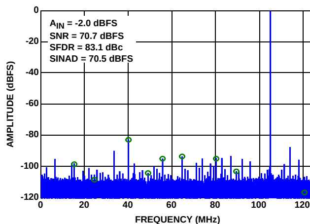
FIGURE 18. SINGLE-TONE SPECTRUM @ 105MHz (250MSPS)
