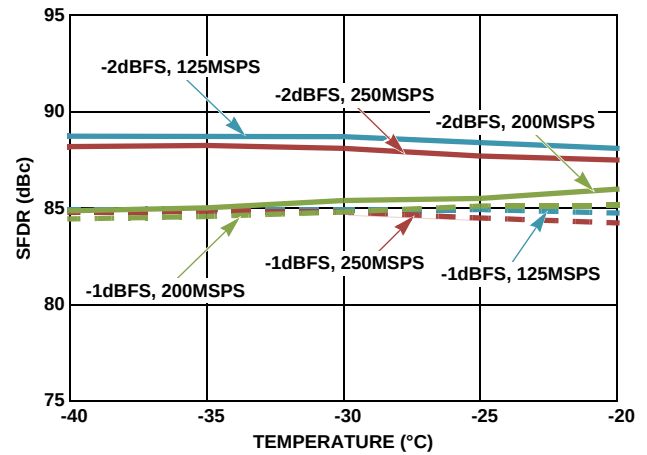
FIGURE 39. TYPICAL SFDR PERFORMANCE vs TEMPERATURE, DEVICE CALIBRATED AT -40^{\circ}\text{C} , f_{\text{IN}} = 105\text{MHz}
