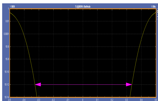
FIGURE 32. SERDES BATHTUB at 4.375Gbps
