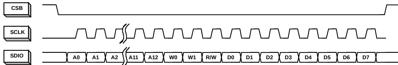
FIGURE 55. LSB-FIRST ADDRESSING
