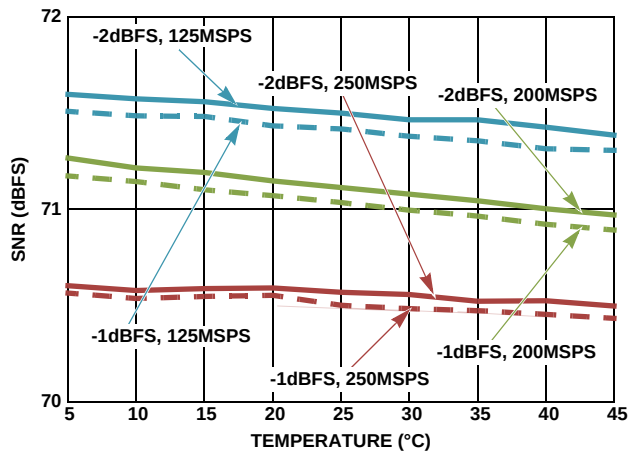
FIGURE 40. TYPICAL SNR PERFORMANCE vs TEMPERATURE, DEVICE CALIBRATED AT +25^{\circ}\text{C} , f_{\text{IN}} = 105\text{MHz}
