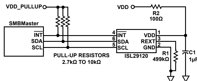
FIGURE 1. TYPICAL APPLICATION
