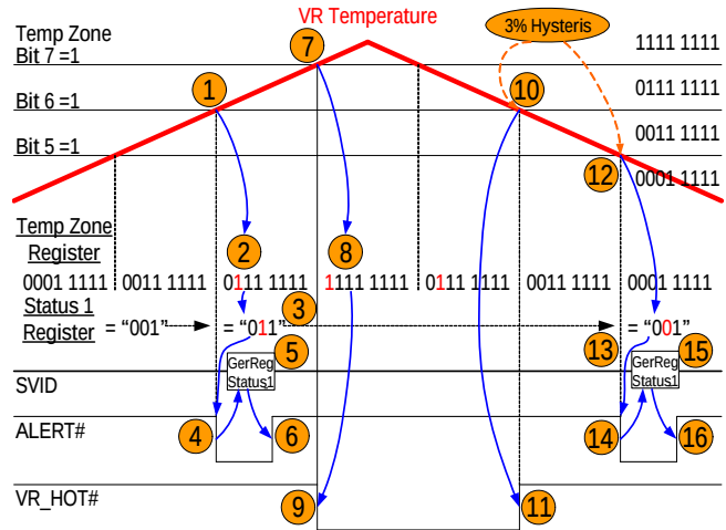
FIGURE 15. VR_HOT#/ALERT# BEHAVIOR
