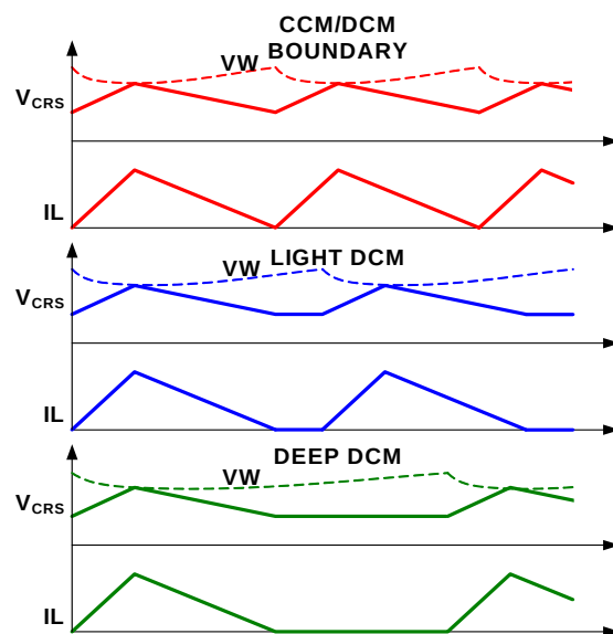
FIGURE 10. PERIOD STRETCHING
