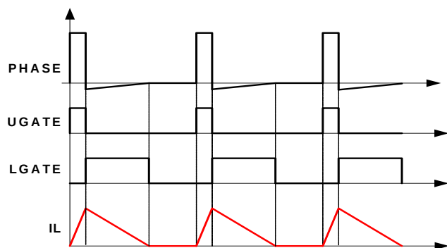
FIGURE 9. DIODE EMULATION
