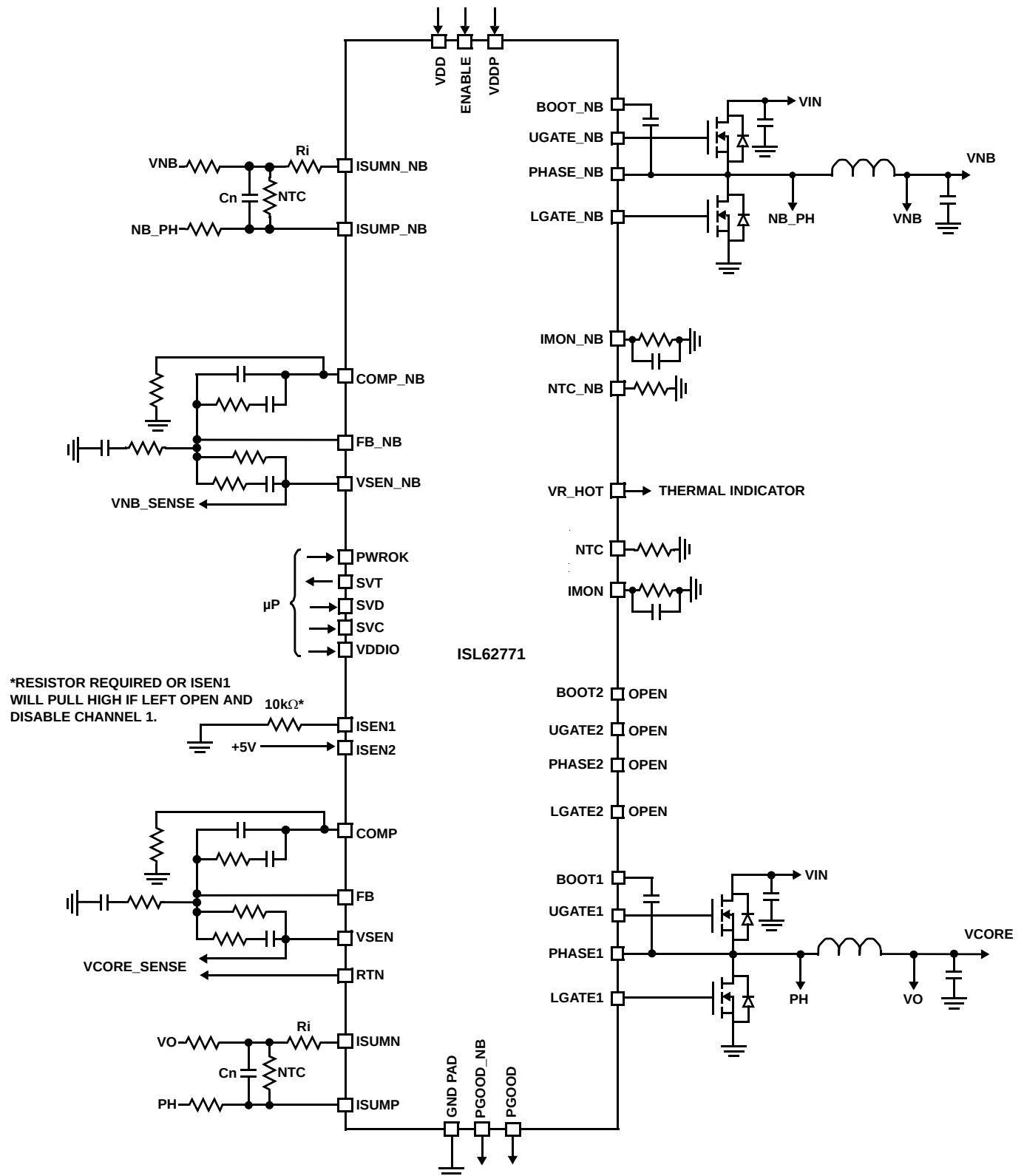
FIGURE 5. TYPICAL APPLICATION CIRCUIT USING INDUCTOR DCR SENSING
