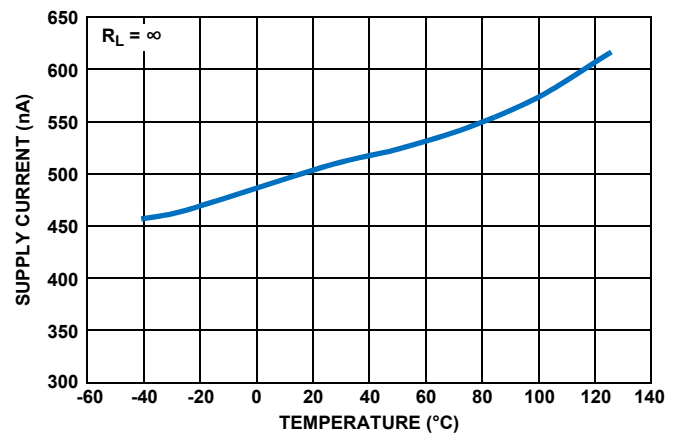
FIGURE 12. SUPPLY CURRENT vs TEMPERATURE, V_+ , GND = \pm 2.5V
