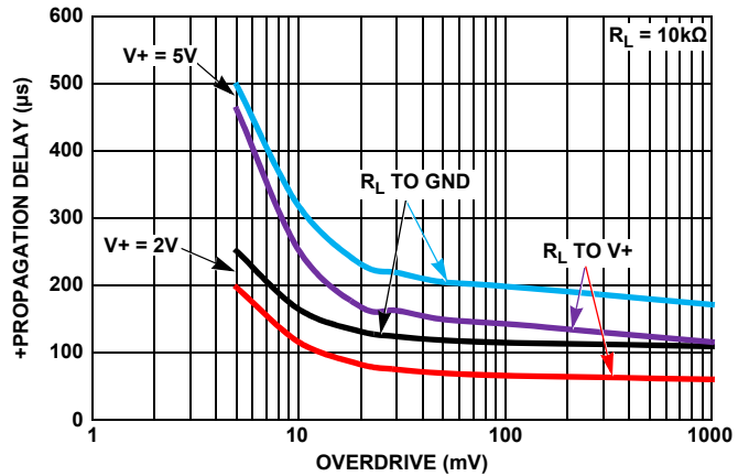
FIGURE 6. PROPAGATION DELAY vs OVERDRIVE (RISING EDGE)
