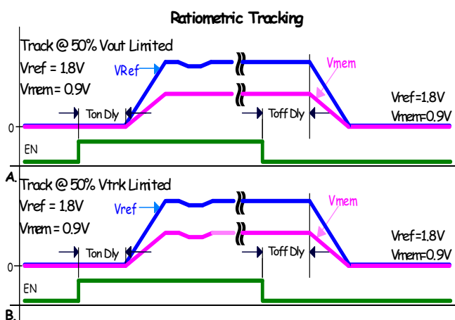
FIGURE 24. RATIOMETRIC TRACKING
