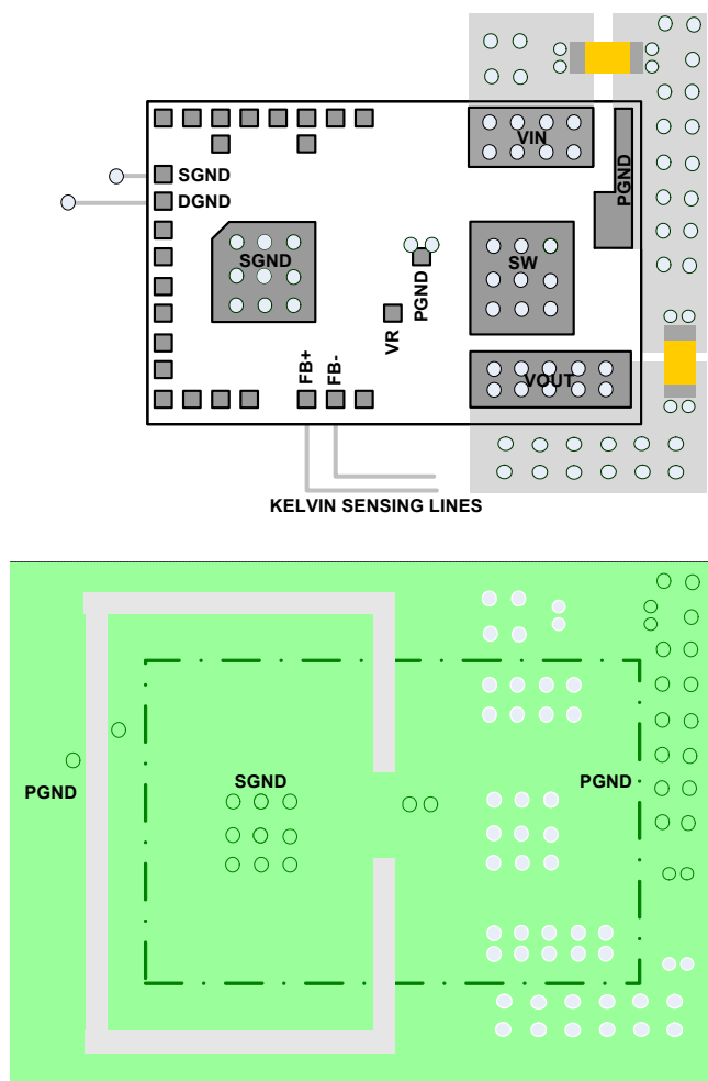
FIGURE 26. RECOMMENDED LAYOUT
