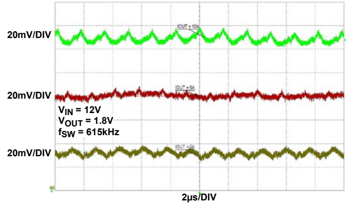
FIGURE 10. V_{OUT} = 1.8\text{V} OUTPUT VOLTAGE RIPPLE
