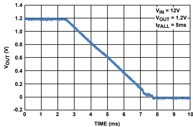
FIGURE 13. SOFT-STOP RAMP-DOWN
