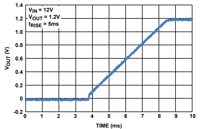
FIGURE 14. SOFT-START RAMP-UP
