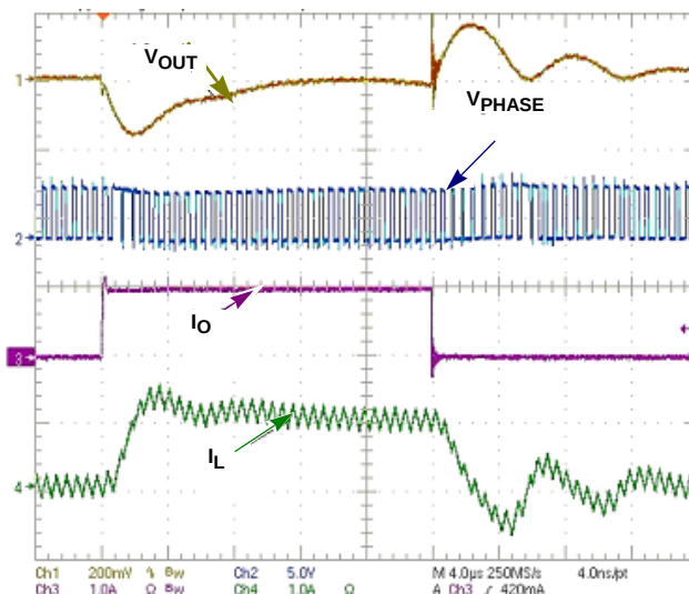
FIGURE 9. LOAD TRANSIENT ( V_{IN} = 3.6V ; V_O = 1.6V ; I_O = 0A TO -1A )
