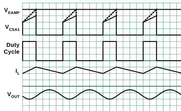
FIGURE 12. PWM OPERATION WAVEFORMS
