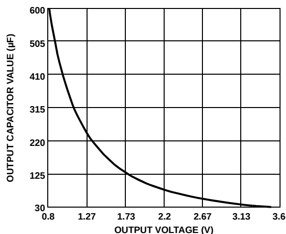
FIGURE 13. THE MAXIMUM CAP vs THE OUTPUT VOLTAGE
