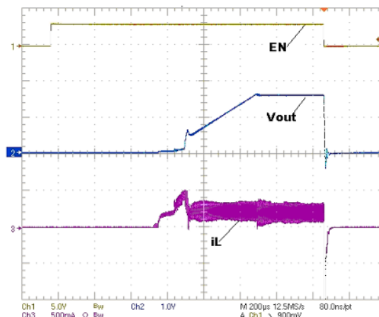
FIGURE 10. SOFT-START
