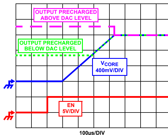
FIGURE 14. SOFT-START WAVEFORMS FOR ISL6323-BASED MULTIPHASE CONVERTER
