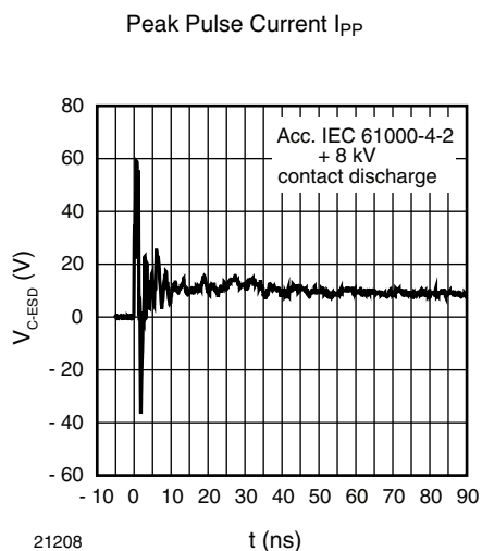
Fig. 7 - Typical Clamping Performance at + 8 kV Contact Discharge (acc. IEC 61000-4-2)
