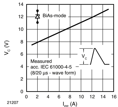
Fig. 6 - Typical Peak Clamping Voltage V_C vs.
