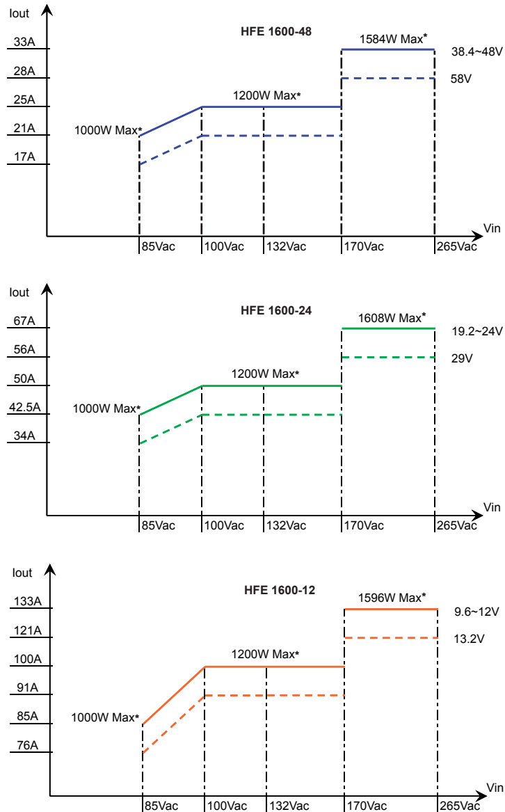
Fig-1 HFE1600 rated output Current and Voltage versus Line Voltage.
