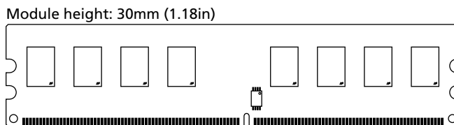
Figure 1: 240-Pin UDIMM (MO-237 R/C E)
