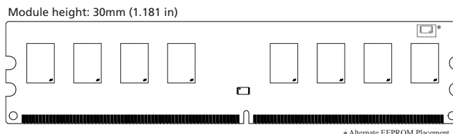
Figure 1: 240-Pin UDIMM (MO-237 R/C D)
