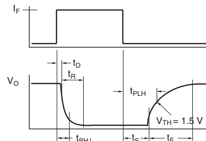
Fig. 6 - Switching Timing
