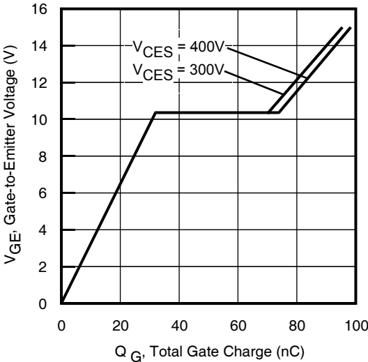
Fig. 19 - Typical Gate Charge vs. V_{GE} I_{CE} = 48A
