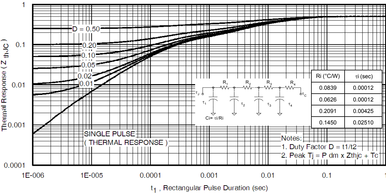
Fig. 20 Maximum Transient Thermal Impedance, Junction-to-Case (IGBT)
