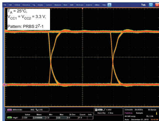
Figure 23. ISO7420FE Typical Eye Diagram at 50 MBPS, 3.3 V Operation
