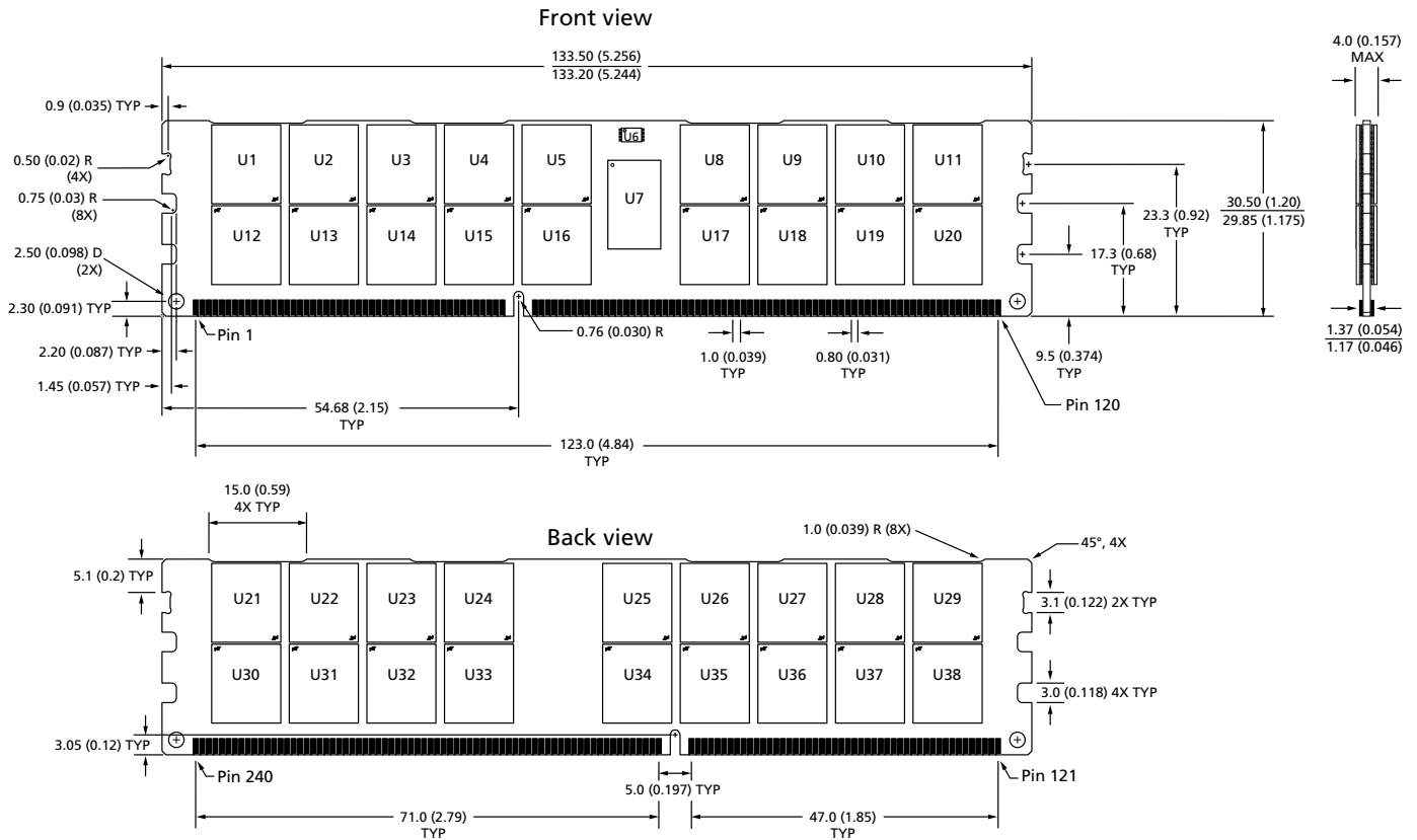
Figure 5: 240-Pin DDR3 RDIMM (R/C J1)
