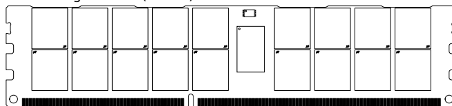
Figure 2: 240-Pin RDIMM (R/C E2)
