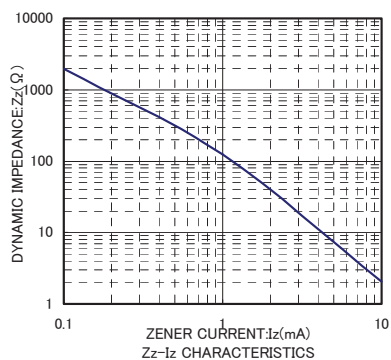
ZENER CURRENT: I_Z (mA) Z_z - I_Z CHARACTERISTICS
