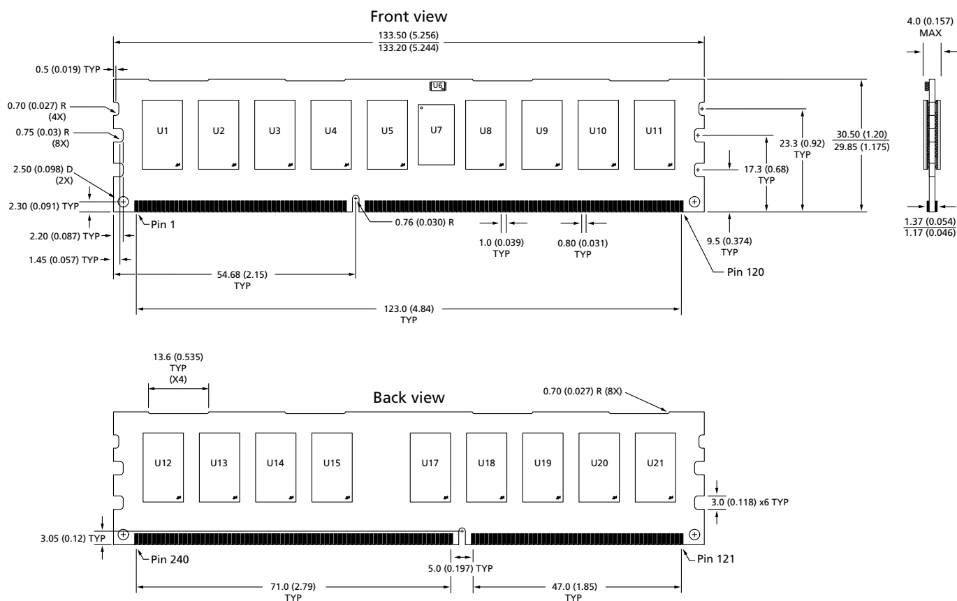
Figure 4: 240-Pin DDR3 RDIMM R/C B (PCB 0693)
