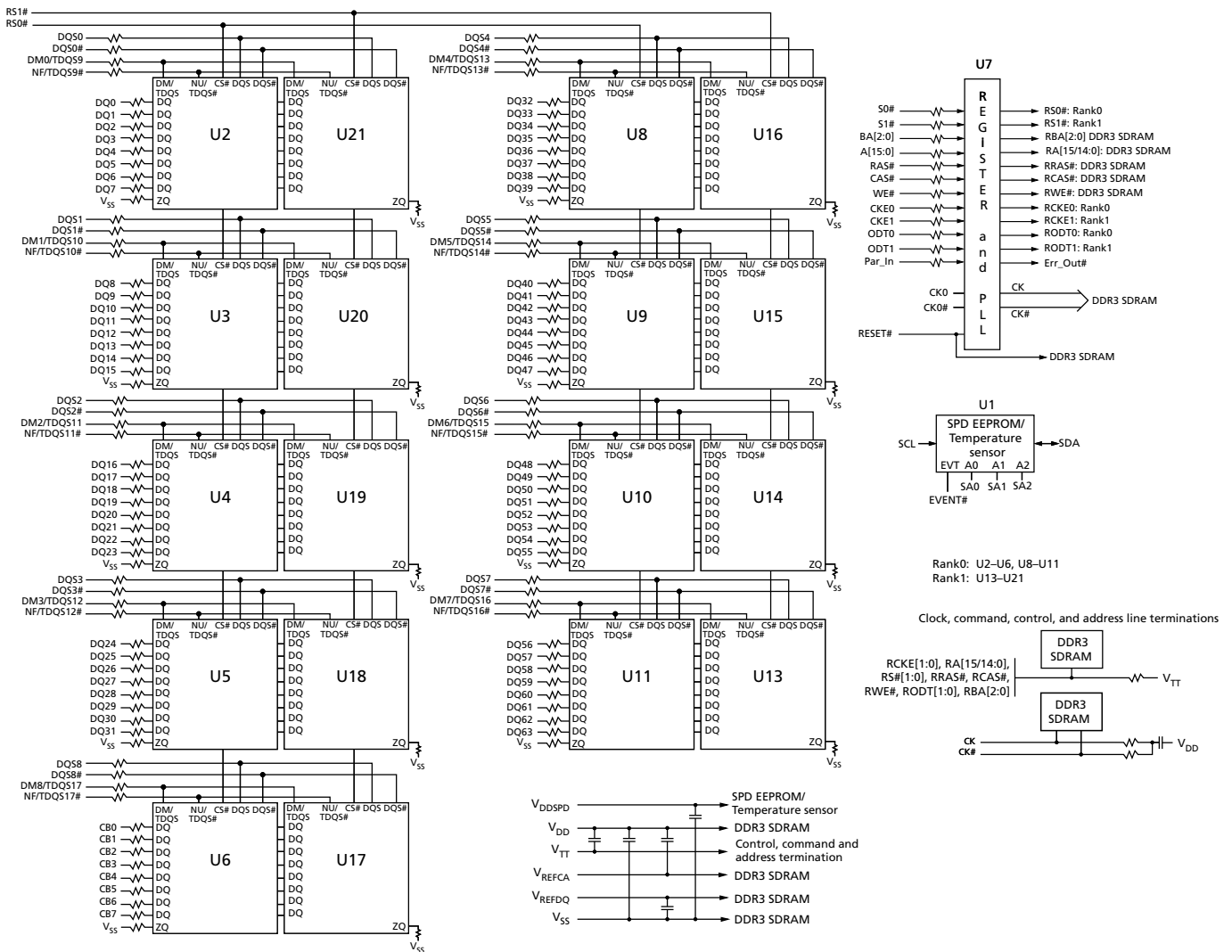
Figure 3: Functional Block Diagram R/C B1(PCB 1164, 1382)
