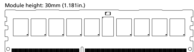
Figure 1: 240-Pin RDIMM (MO-269 R/C B, R/C B1)
