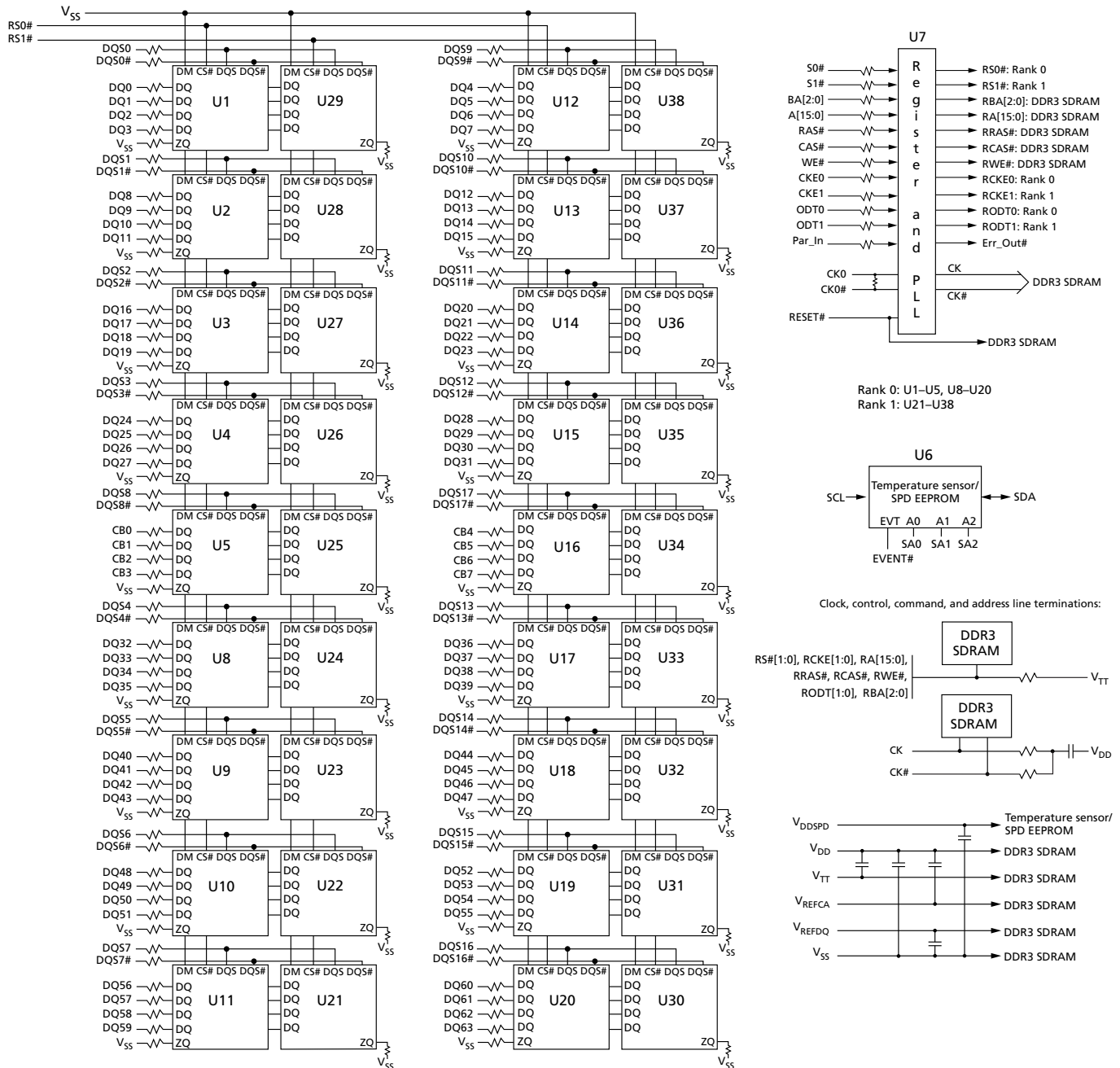
Figure 3: Functional Block Diagram (R/C J1)
