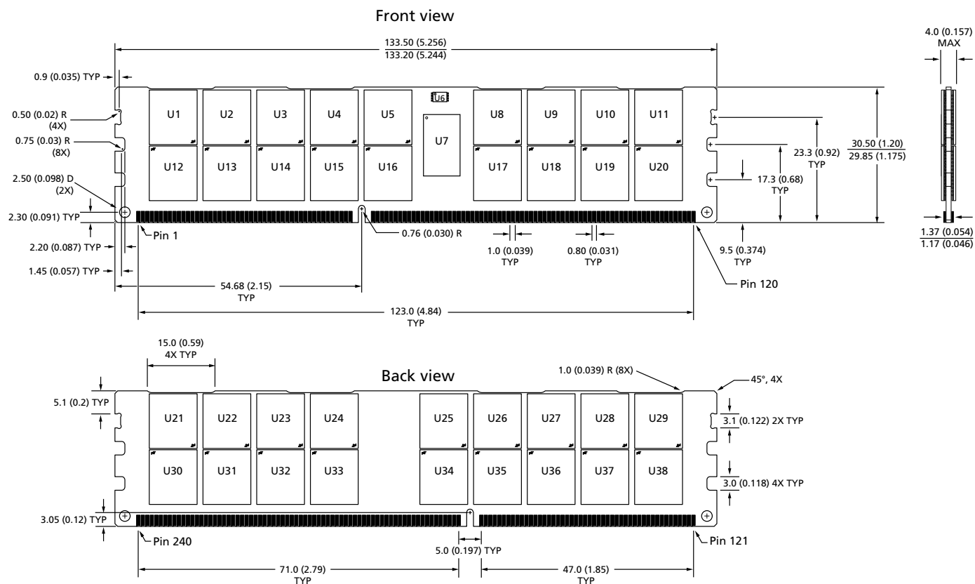
Figure 5: 240-Pin DDR3 RDIMM (R/C J1)
