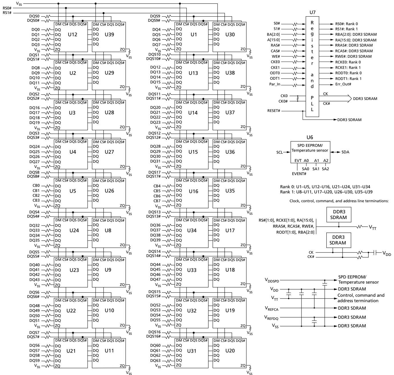
Figure 4: Functional Block Diagram (R/C E2)
