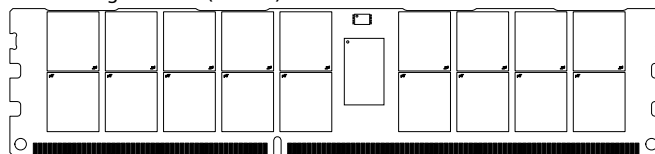
Figure 2: 240-Pin RDIMM (MO-269 R/C E2)
