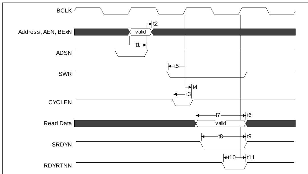
Figure 21. Synchronous Read Cycle – VLBSN = 0
