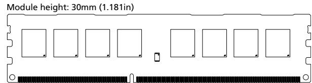
Figure 1: 240-Pin UDIMM (MO-269 R/C A)
