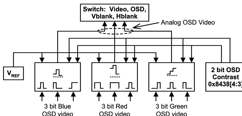
Figure 13. Block Diagram of OSD DACs
