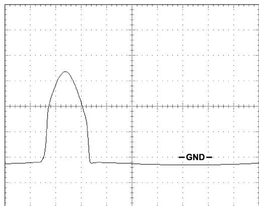
Figure 3. Deflection Horizontal Blanking
