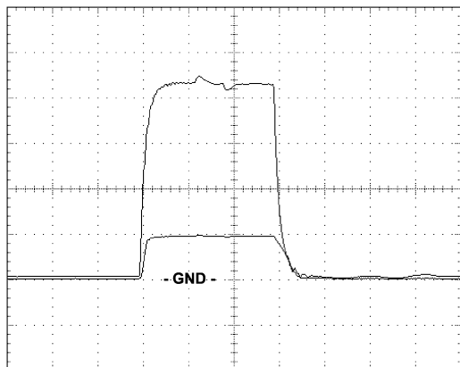
Figure 1. Logic Horizontal Blanking
