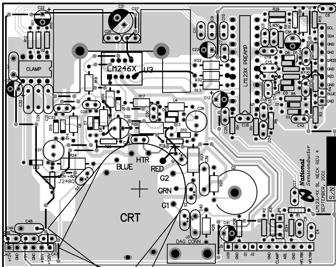
Figure 10. LM123x/LM124x-LM246x Demo Board Layout
