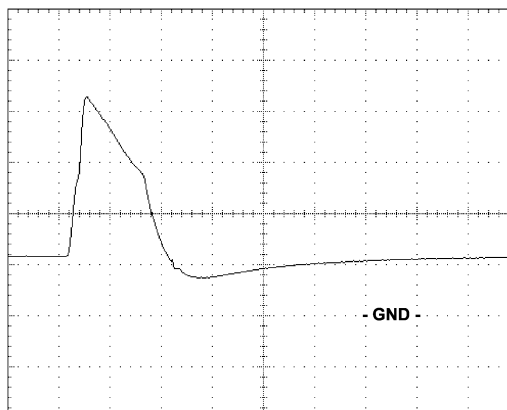
Figure 4. Deflection Vertical Blanking
