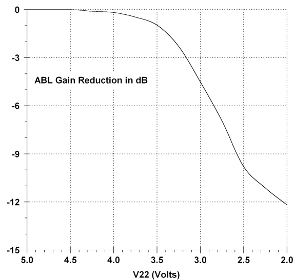
Figure 7. ABL Gain Reduction Curve
