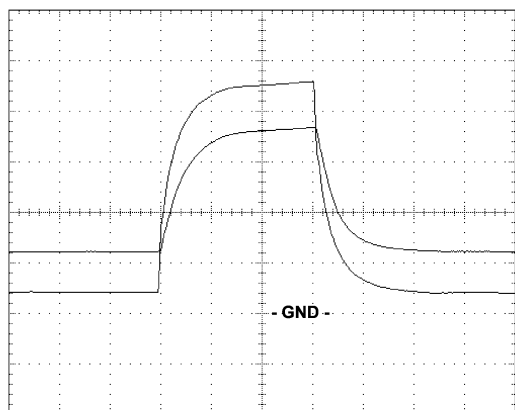
Figure 5. Logic Clamp Pulse
