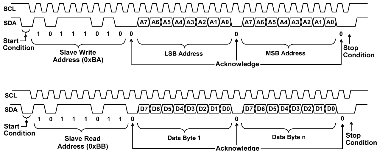
Figure 23. I 2 C Compatible Read Sequence
