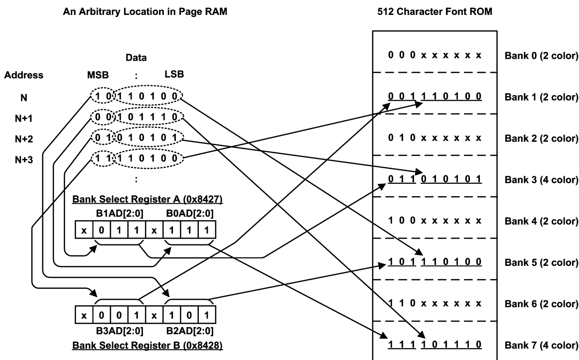
Figure 12. Bank Addressing
