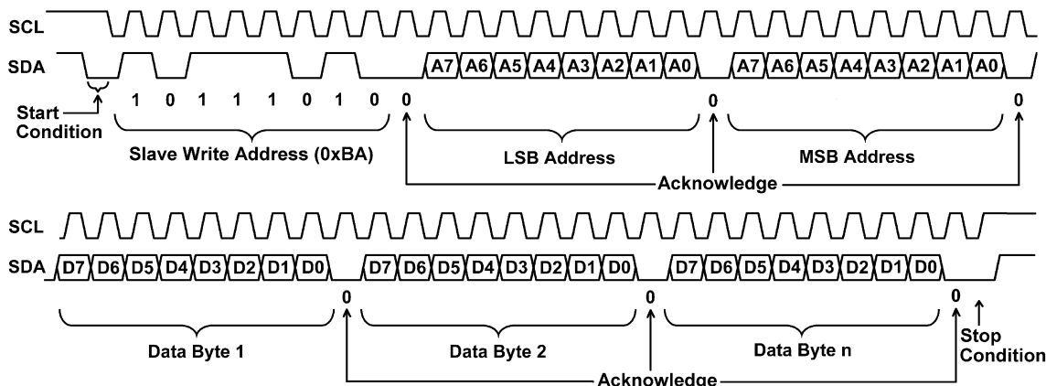
Figure 22. I 2 C Compatible Write Sequence
