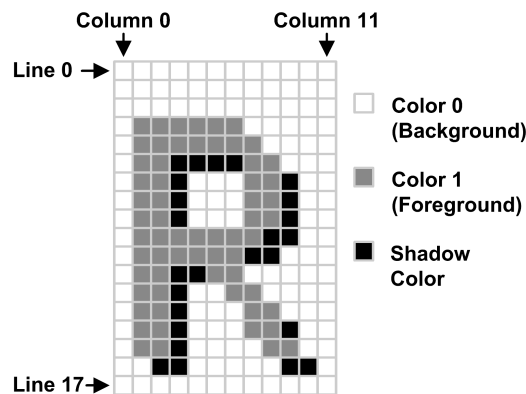
Figure 27. Operation of the Shadow Feature
