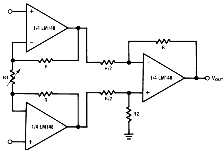
Figure 20. Low Cost Instrumentation Amplifier
