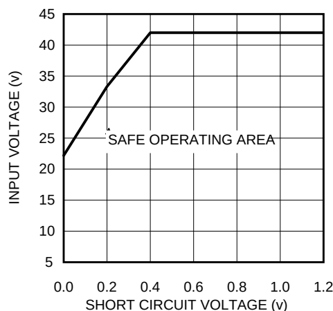
Figure 13. SOA
