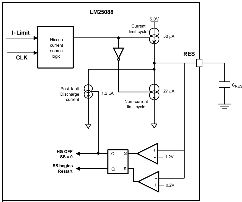
Figure 21. Current Limit Restart Circuit
