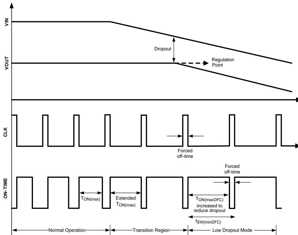
Figure 18. Dropout Voltage Reduction using Dynamic Frequency Control
