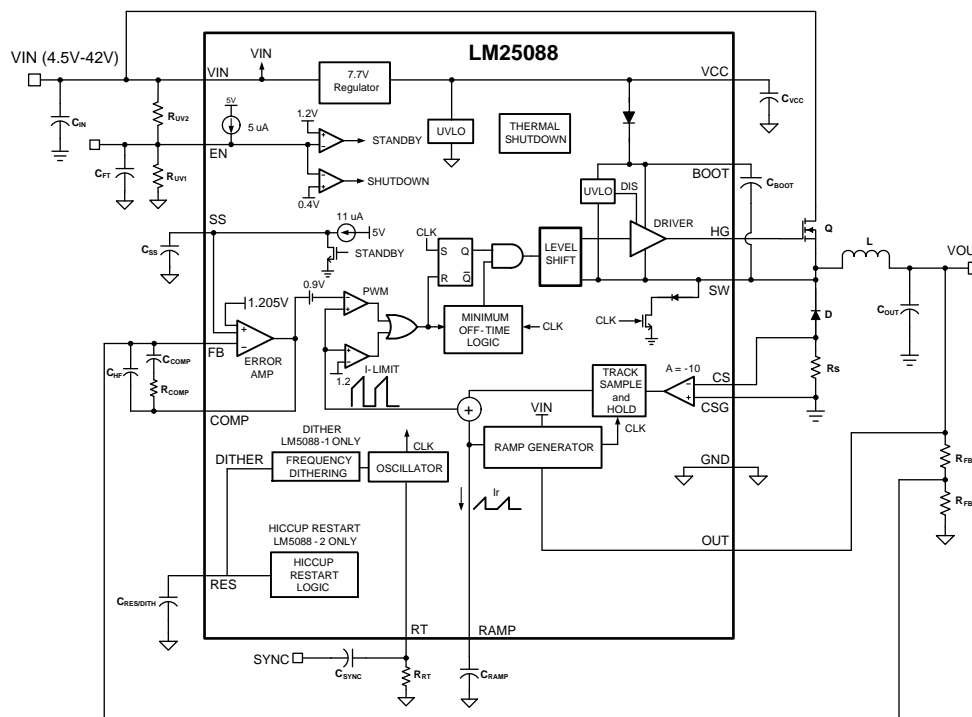
Figure 15. Block Diagram
