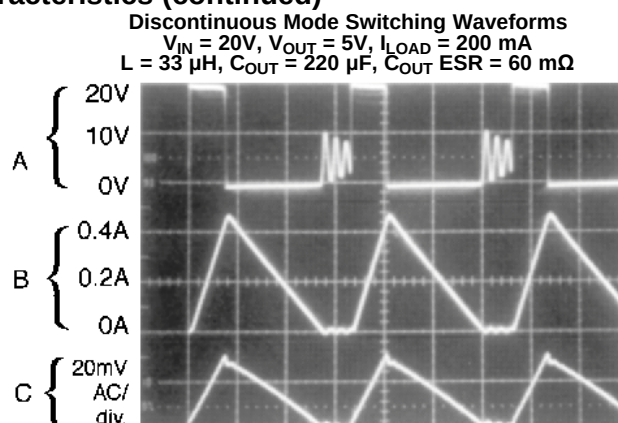
A: Output Pin Voltage, 10V/div. B: Inductor Current 0.2A/div. C: Output Ripple Voltage, 20 mV/div.
