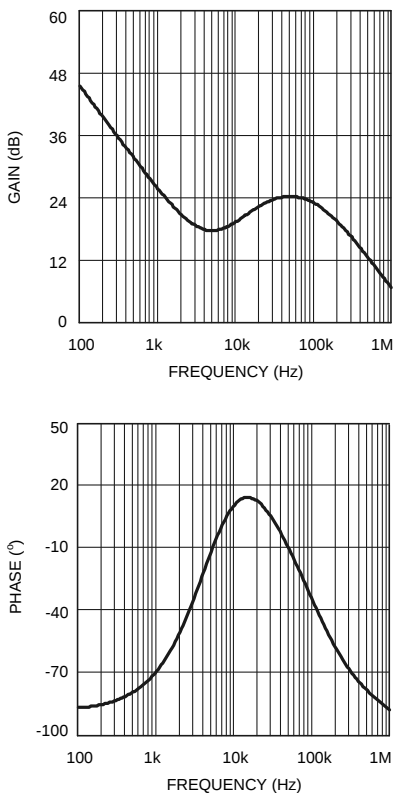
Figure 37. Error Amp. Gain and Phase
