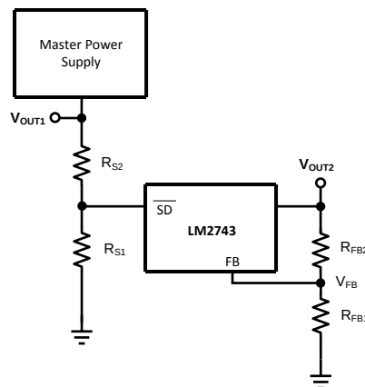
Figure 26. Sequencing Circuit
