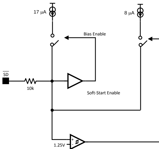
Figure 28. \overline{\text{SD}} Pin Logic
