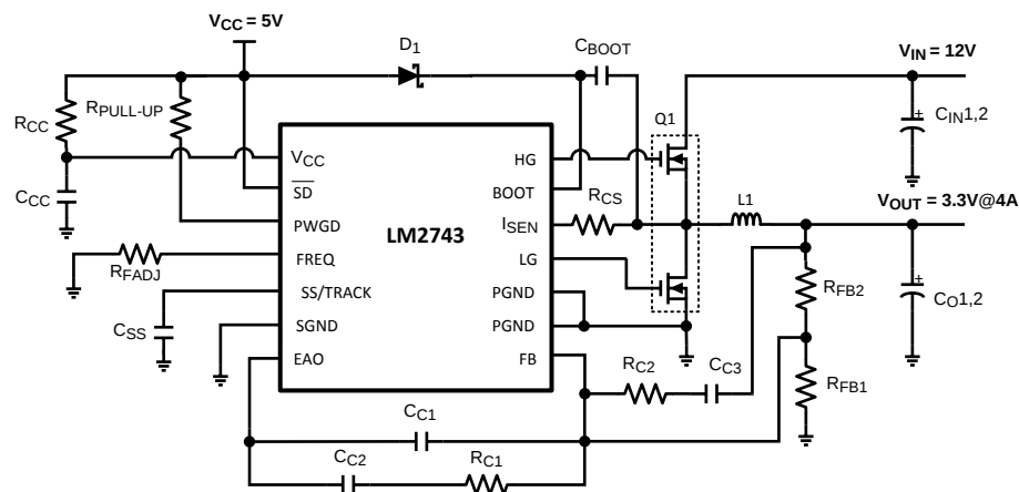
Figure 41. 12V to 3.3V @ 4A, f_{SW} = 300\text{kHz}
