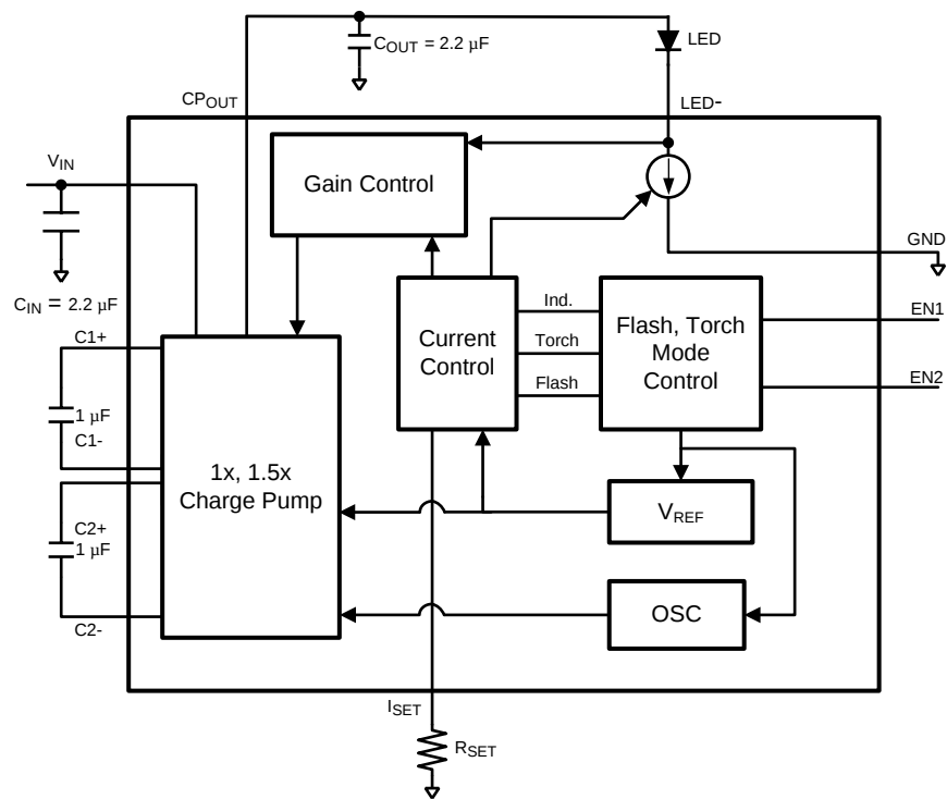
LM2758 Block Diagram
