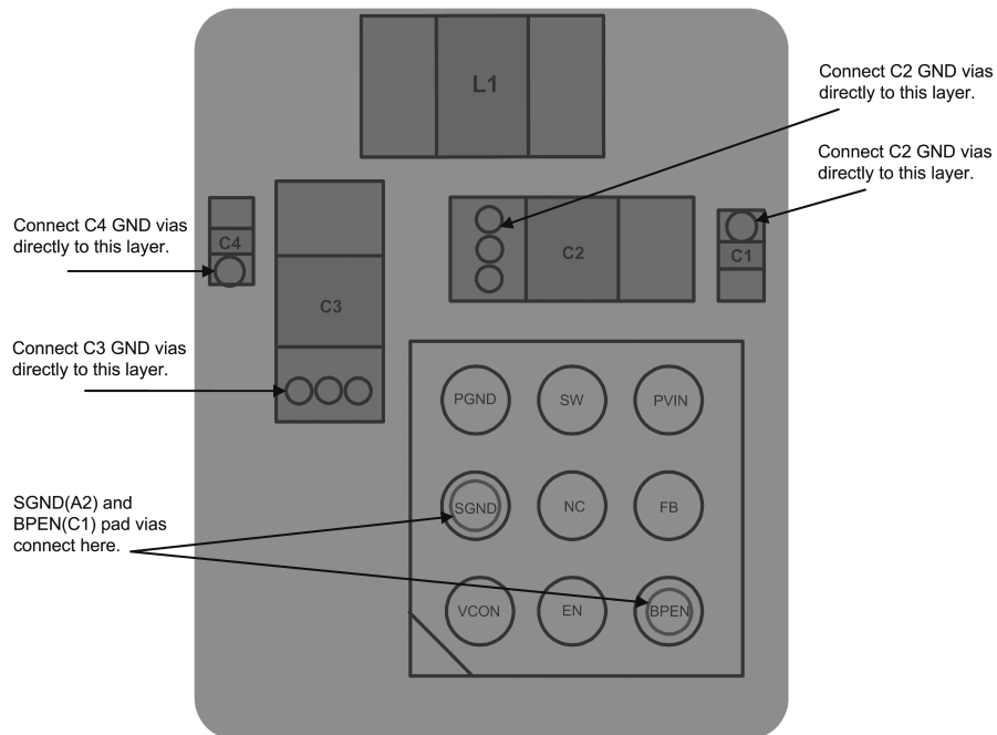
Figure 37. Board Layer 4 – System GND Plane
