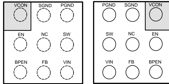
Figure 1. 9-Bump Thin DSBGA Package Large Bump (0.4 mm Pitch) Package Number YFQ0009
