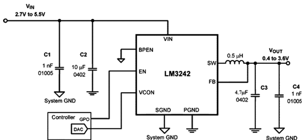
Figure 32. Simplified LM3242 RF Evaluation Board Schematic
