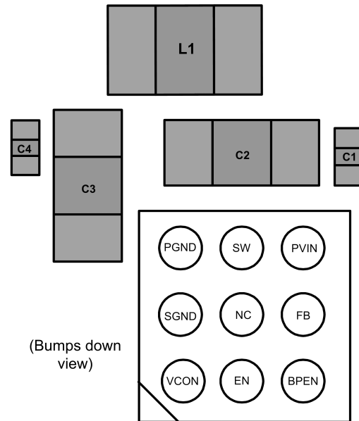
Figure 33. LM3242 Recommended Parts Placement (Top View)
