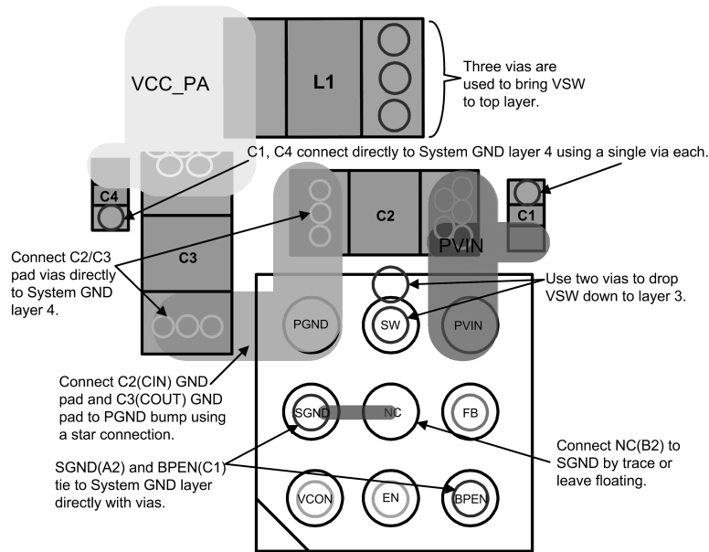
Figure 34. Board Layer 1 – PVIN and PGND Routing
