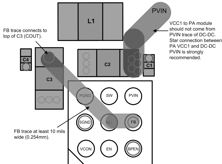
Figure 35. Board Layer 2 – FB and PVIN Routing
