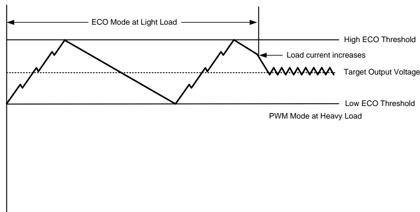
Figure 31. Operation in ECO Mode and Transfer to PWM Mode
