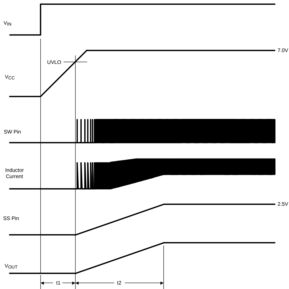
Figure 12. Startup Sequence
