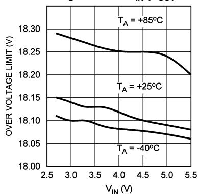
Over Voltage Limit vs V_{IN} ( V_{OUT} Falling)
