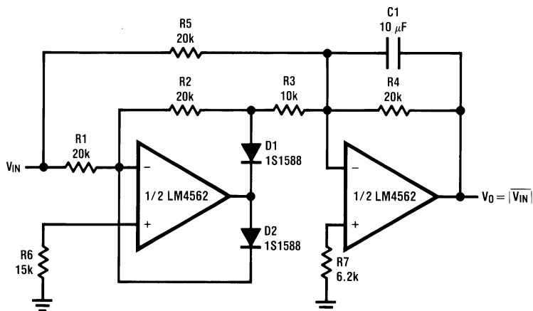
Figure 122. AC/DC Converter
