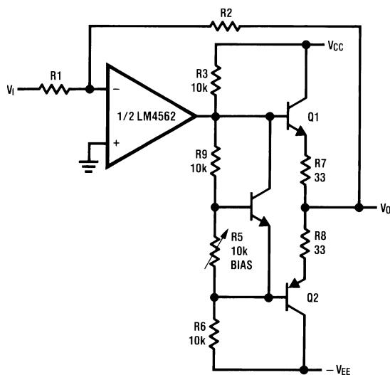
Figure 124. Line Driver
