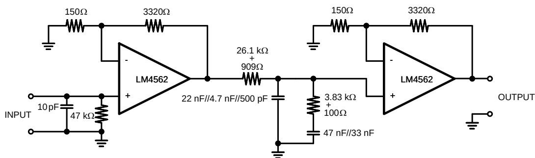
Figure 1. Passively Equalized RIAA Phono Preamplifier
