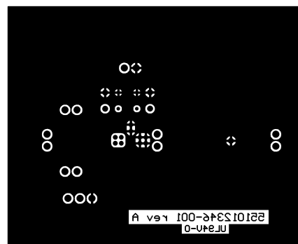
Figure 38. Bottom Layer
