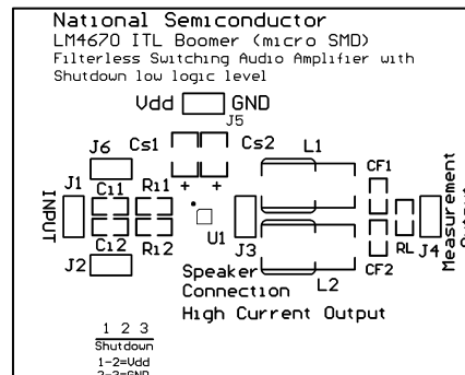
Figure 34. Silk Screen
