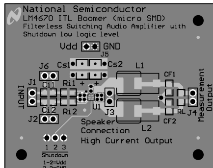
Figure 33. Composite View
