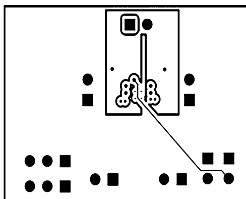
Figure 35. Mid 2 Layer
