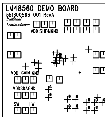
Figure 35. Drill Drawing
