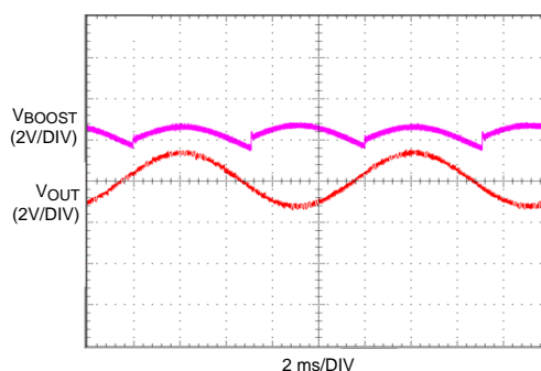
Figure 28. Class H Operation
