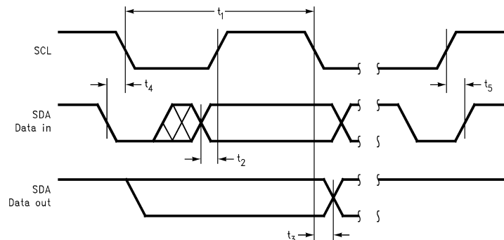
Figure 51. I²C Timing Diagram
