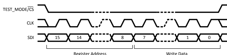
Figure 4-6. SPI Write Transaction
