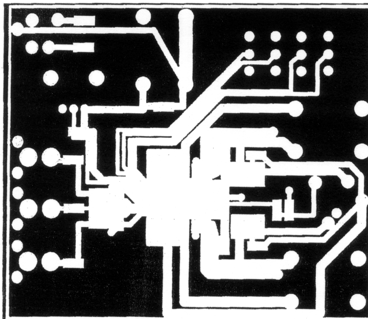
Figure 49. Inner Layer (2)
