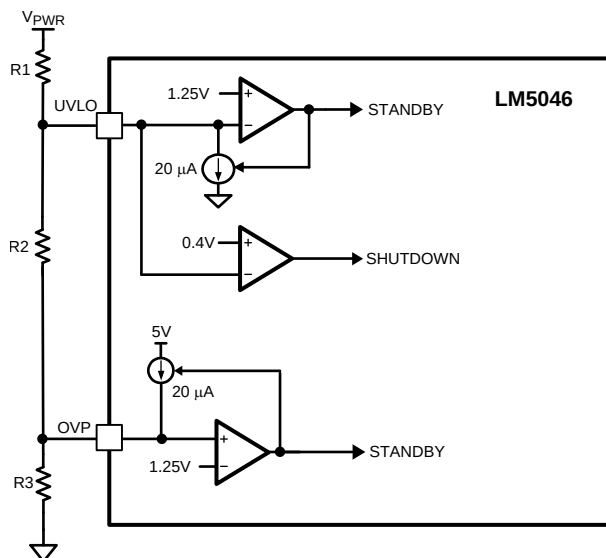
Figure 28. UVLO/OVP Divider
