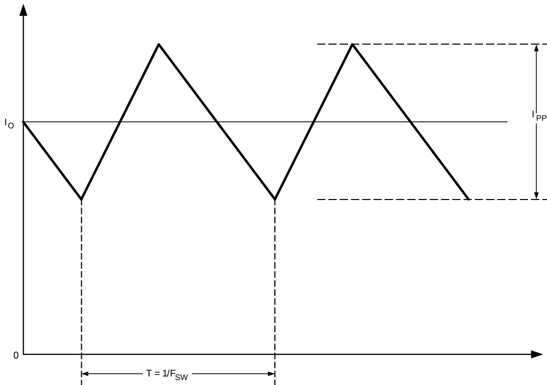
Figure 23. Inductor Current
