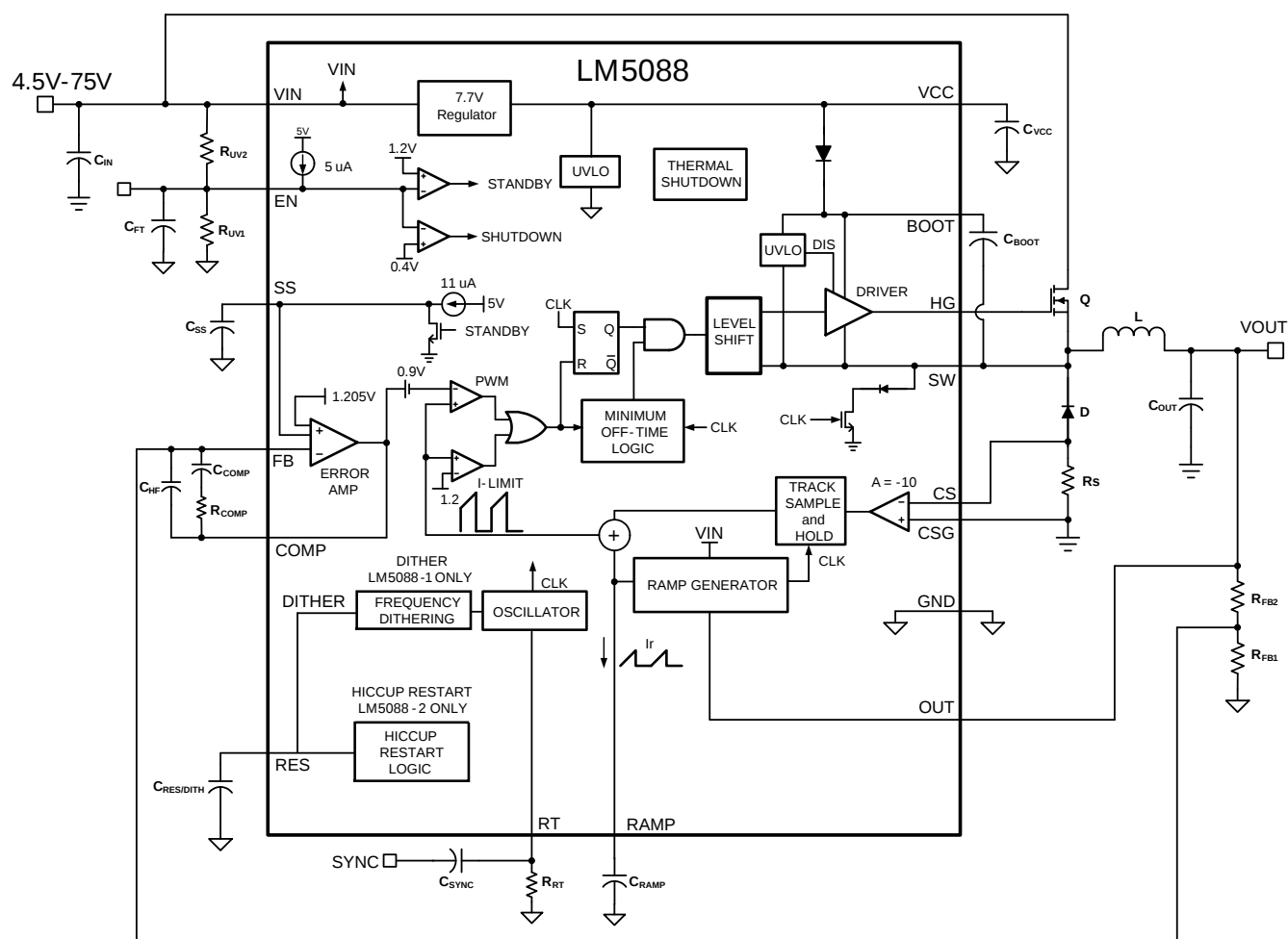
Figure 15. Block Diagram
