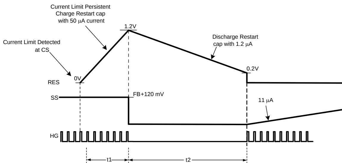
Figure 22. Current Limit Restart Timing Diagram
