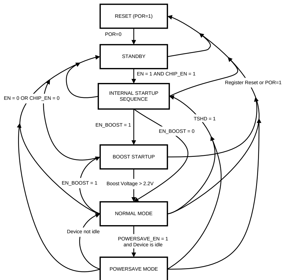
Figure 16. Startup Sequence
