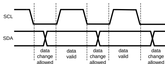
Figure 24. Data Validity Diagram
