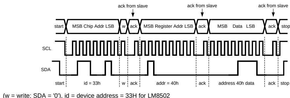
Figure 27. Write Cycle
