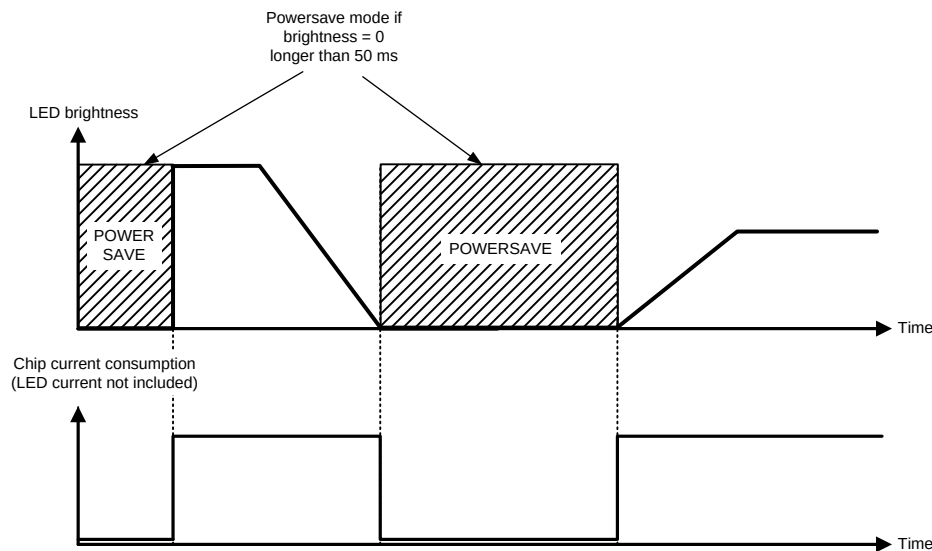
Figure 23. The Effect of Power-Save Mode During a Lighting Sequence
