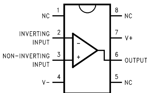
Figure 1. 8-Pin SOIC (Top View)
