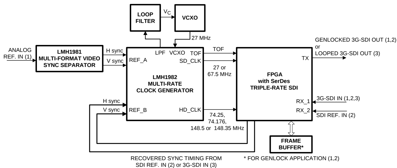
Figure 17. Triple-Rate SDI Loop-through
