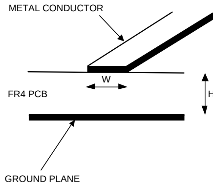
Figure 95. Microstrip Configuration
