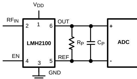
Figure 92. Differential Application
