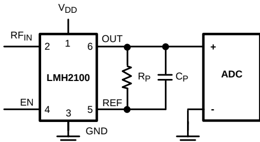
Figure 91. Single Ended
