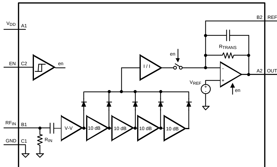
Figure 4. LMH2100
