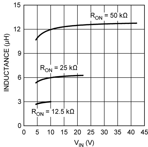
Figure 26. Inductor selection for V_{OUT} = 0.8\text{V}
