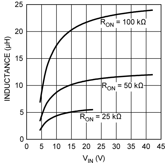
Figure 25. Inductor selection for V_{OUT} = 3.3\text{V}
