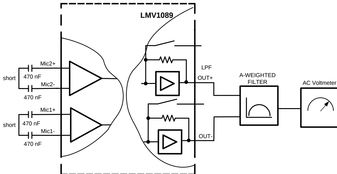
Figure 36. Noise Measurement Setup
